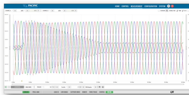
Waveform Example of Inductive Motor Emulation: 400Hz, 55A
