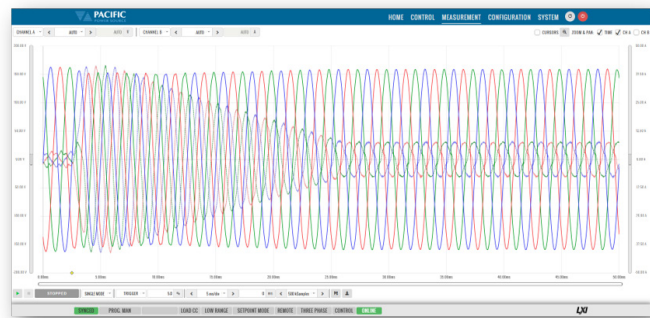
Waveform Example: Inductive Motor Emulation: 400Hz, 55A (overload capability from 42A)
